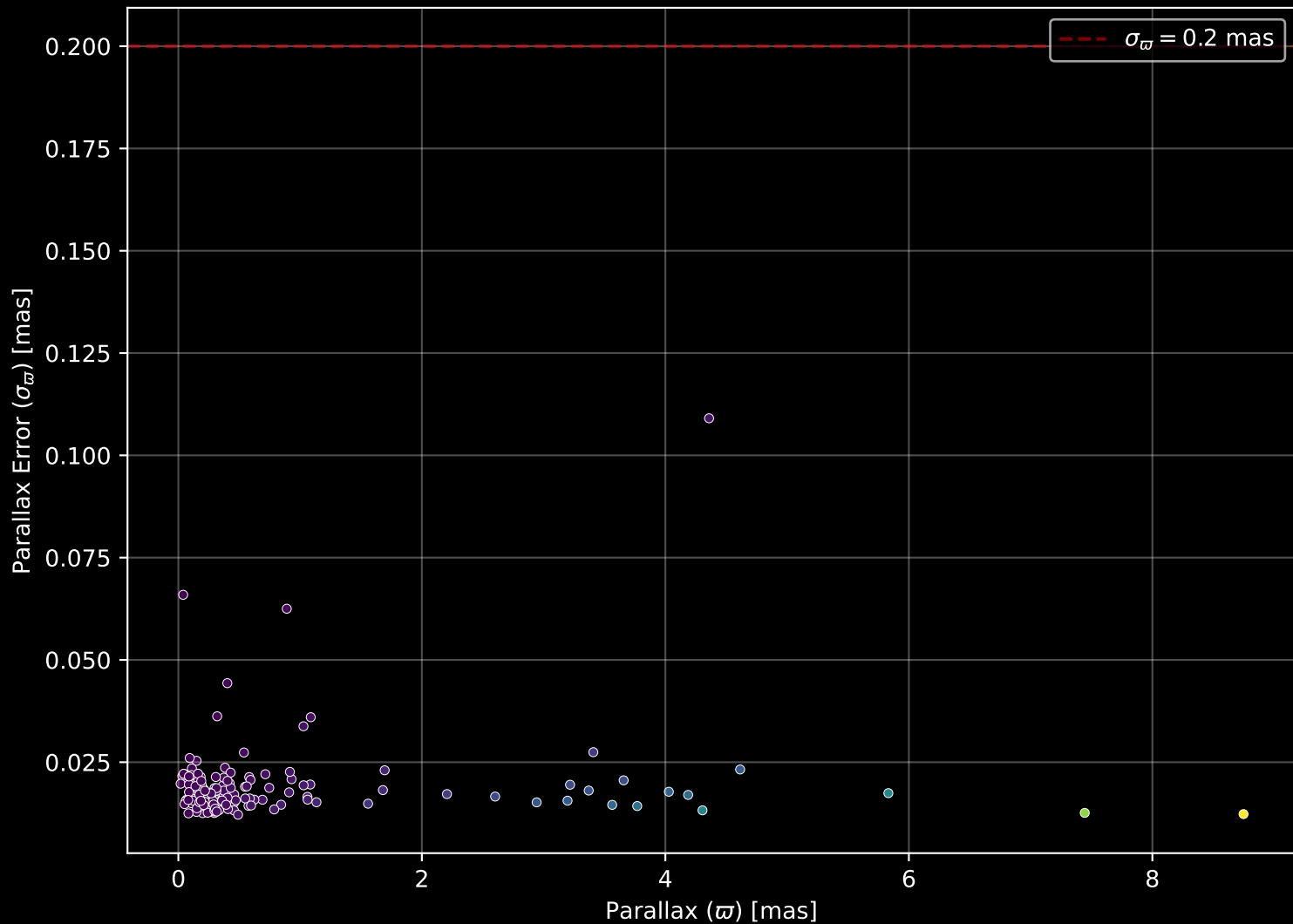
APOGEE DR17 Field: [225-12] Parallax Quality (n= 152)
