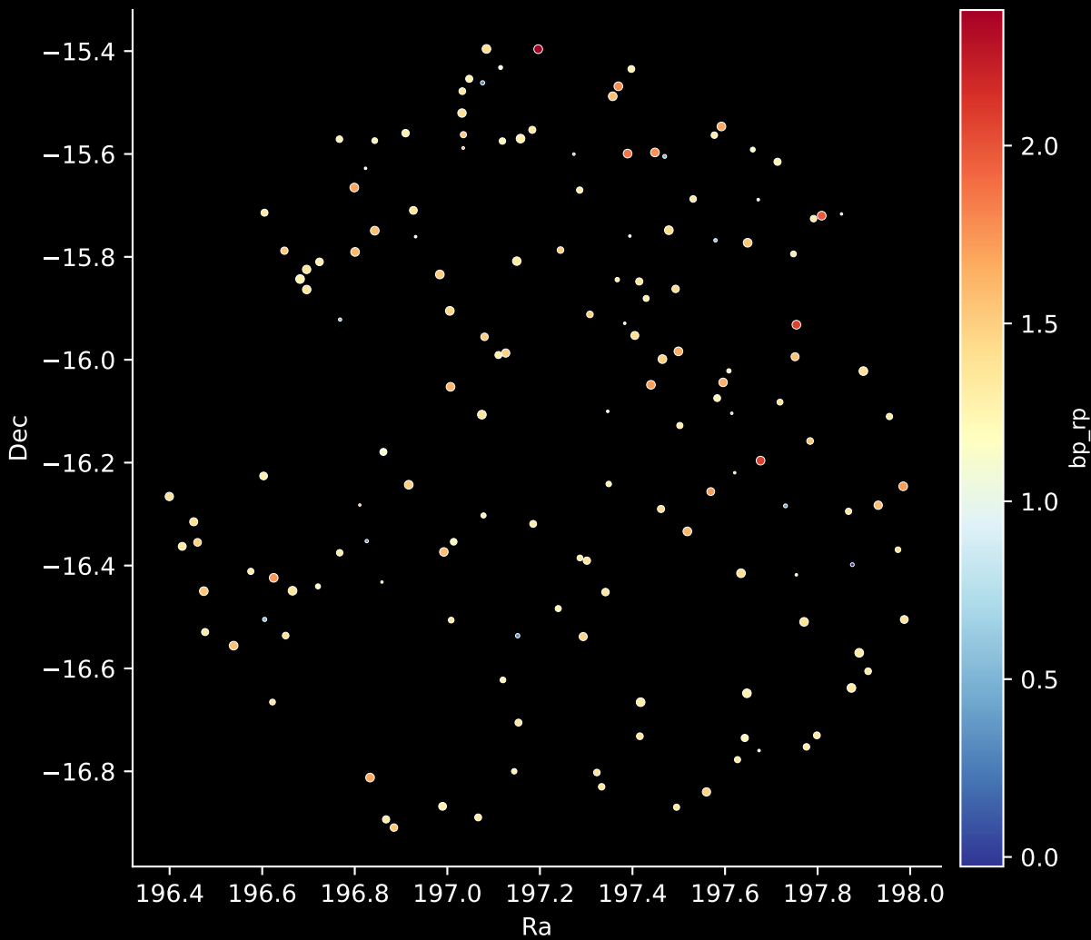
APOGEE DR17 Field: [225-12] Stars: 152
