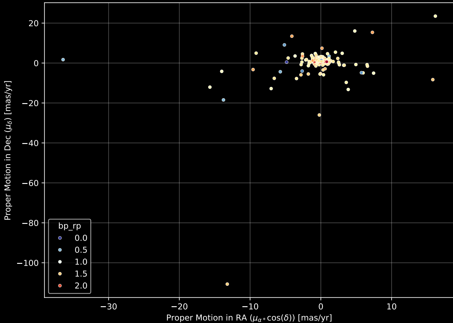
APOGEE DR17 Field: [225-12] Proper Motion Diagram (n= 152)
