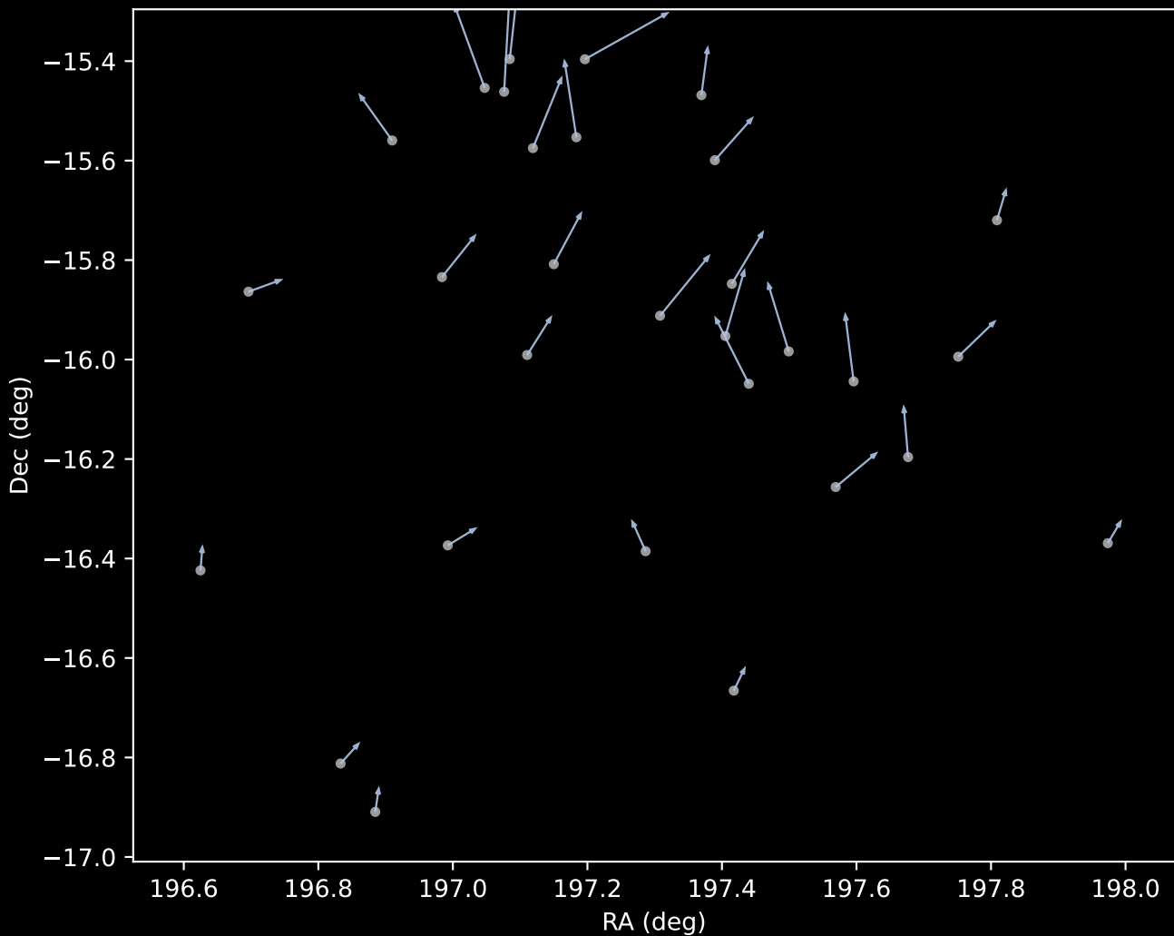
APOGEE DR17 Cluster 1 Proper Motion Vectors (n=30)
