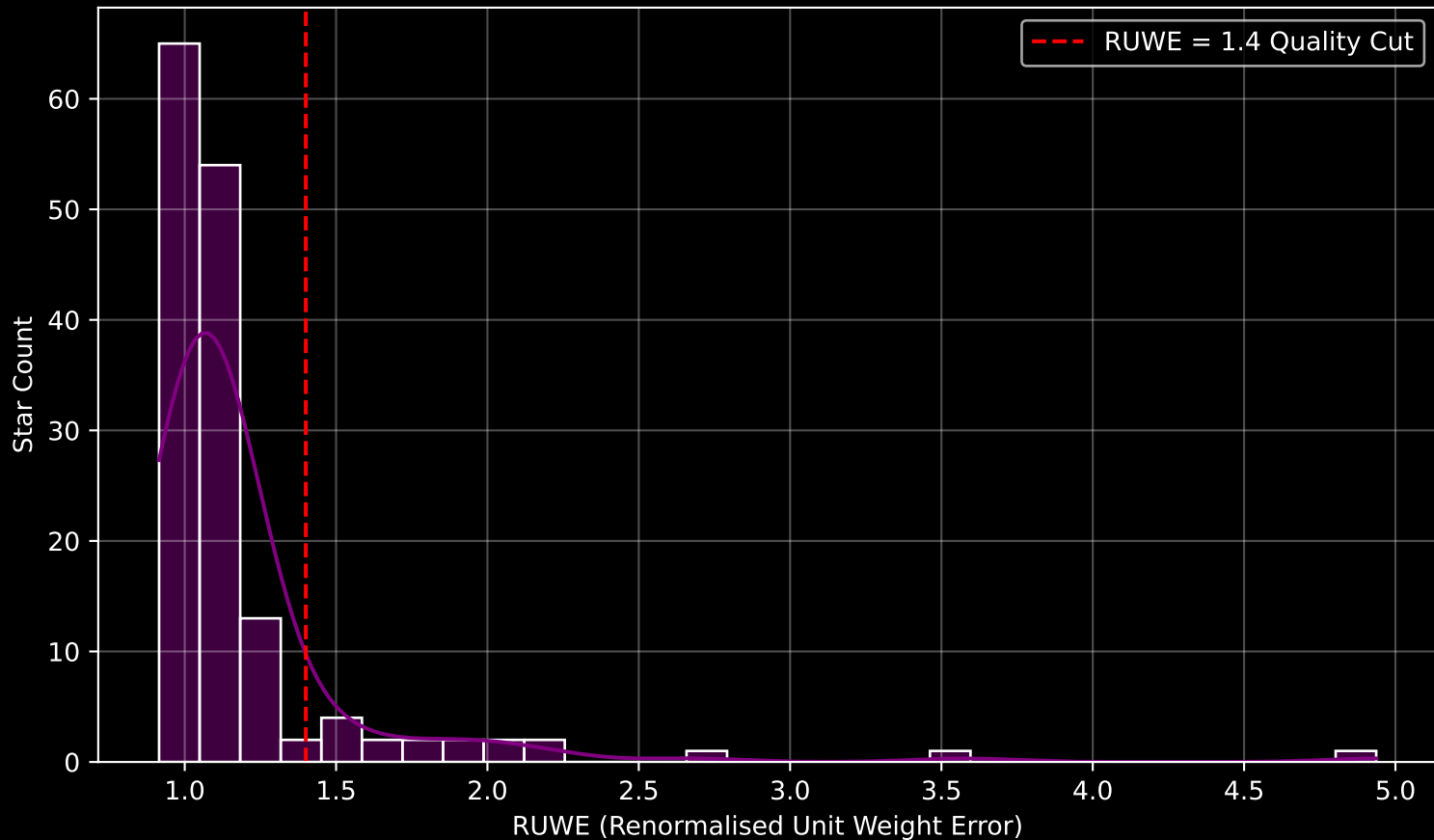
GAPOGEE DR17 Field [225-12] RUWE Distribution (n= 151)
