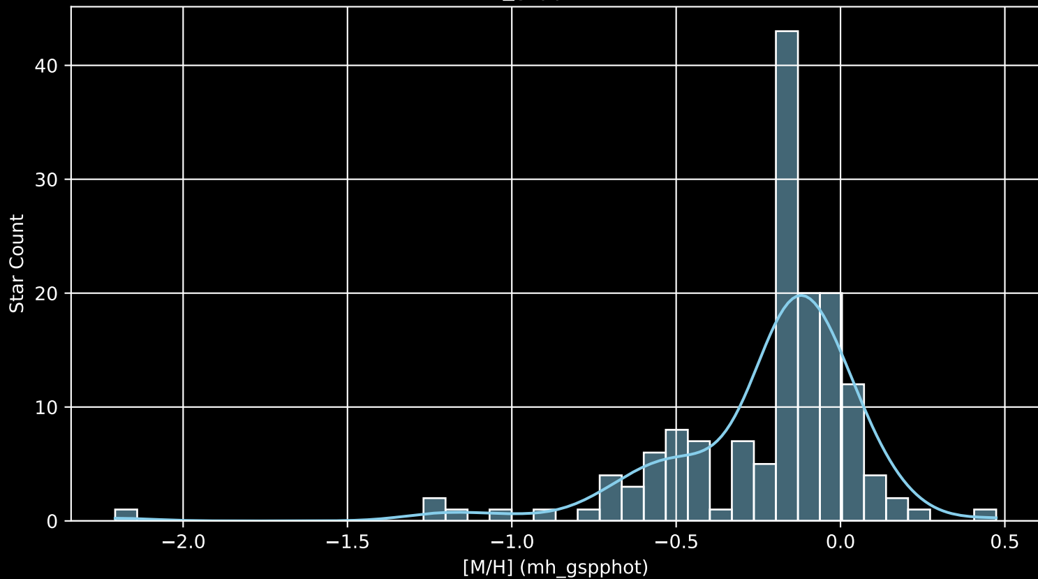
APOGEE DR17 Field: [225-12 [M/H] (mh_gspphot) (n= 151)
