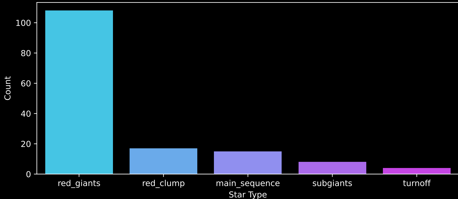
APOGEE DR17 Field: [225-12] Count plot of Star Type
